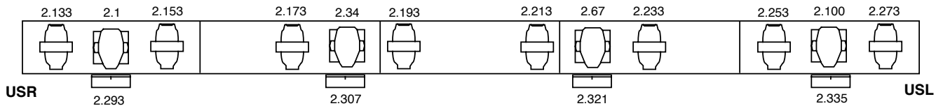
Upstage Truss - Universe 2
