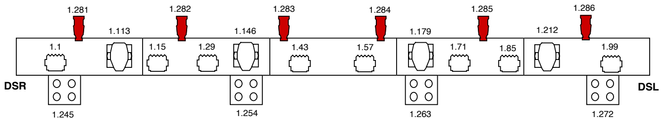
Downstage Truss - Universe 1
